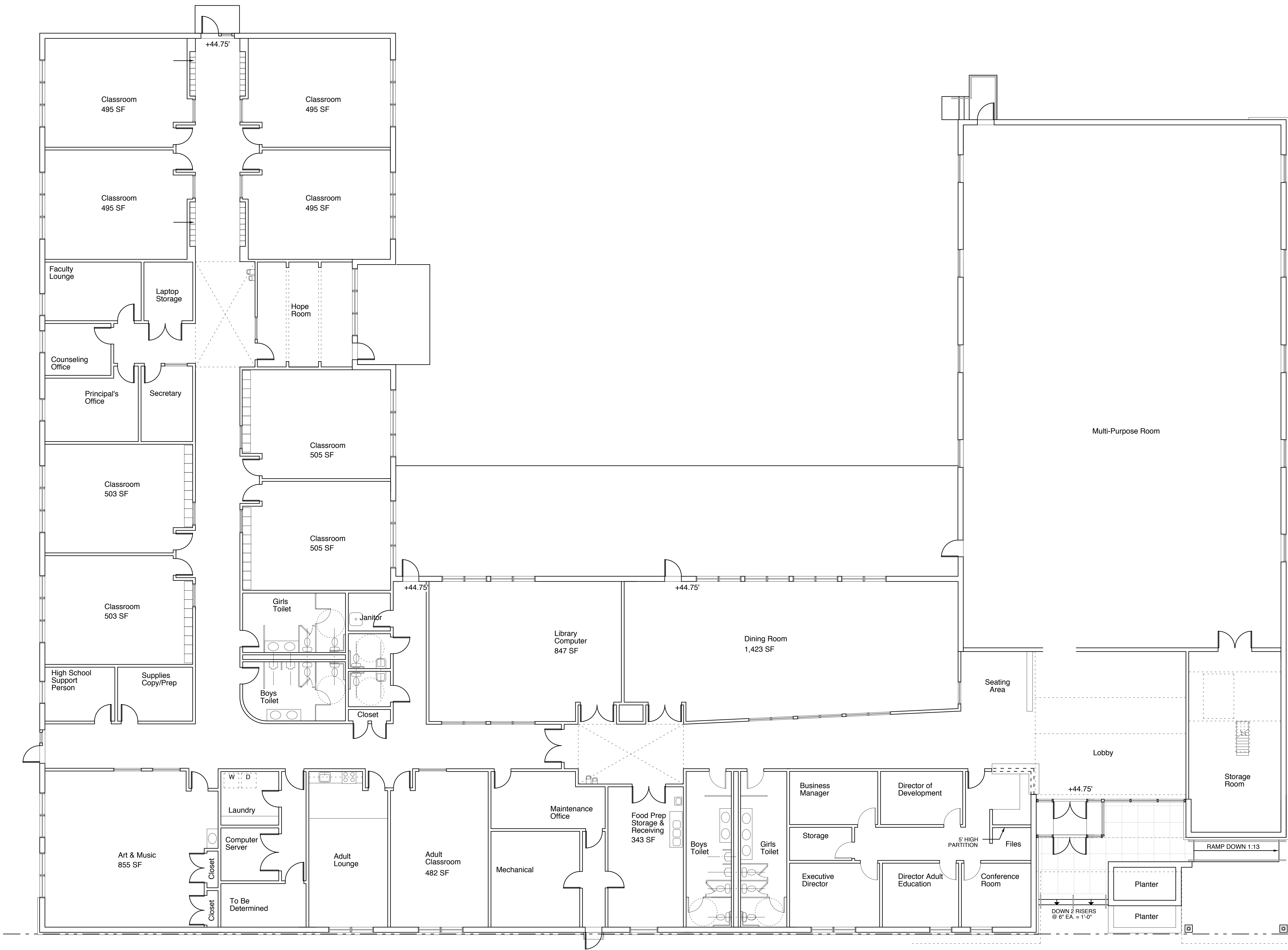
1 A-1 First Floor Plan - 23,575 sf
